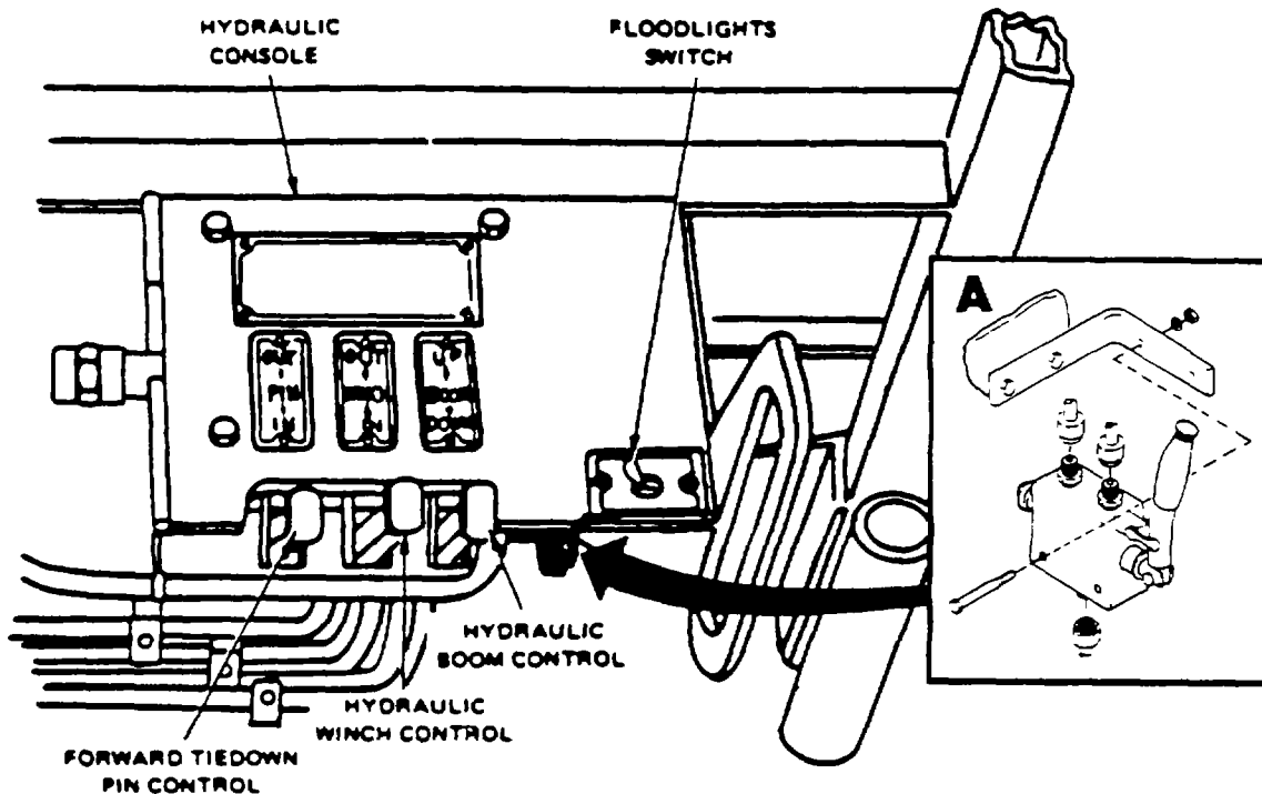
Figure 2-1. Hydraulic Controls
