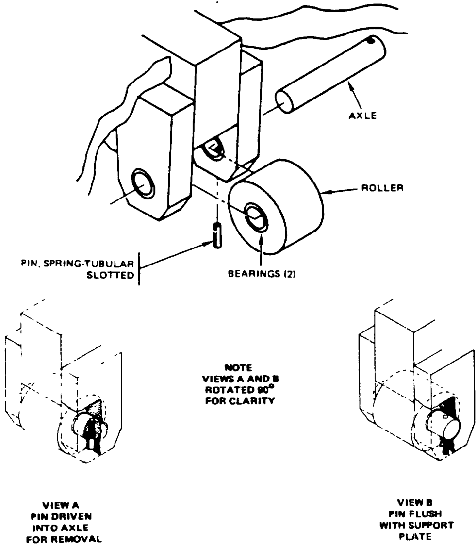
Figure 4-1. Axle and Roller. Disassembly for Lubrication.
