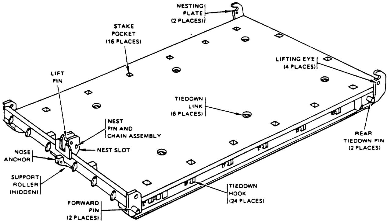
Figure 1-1. Cargo Pallet
