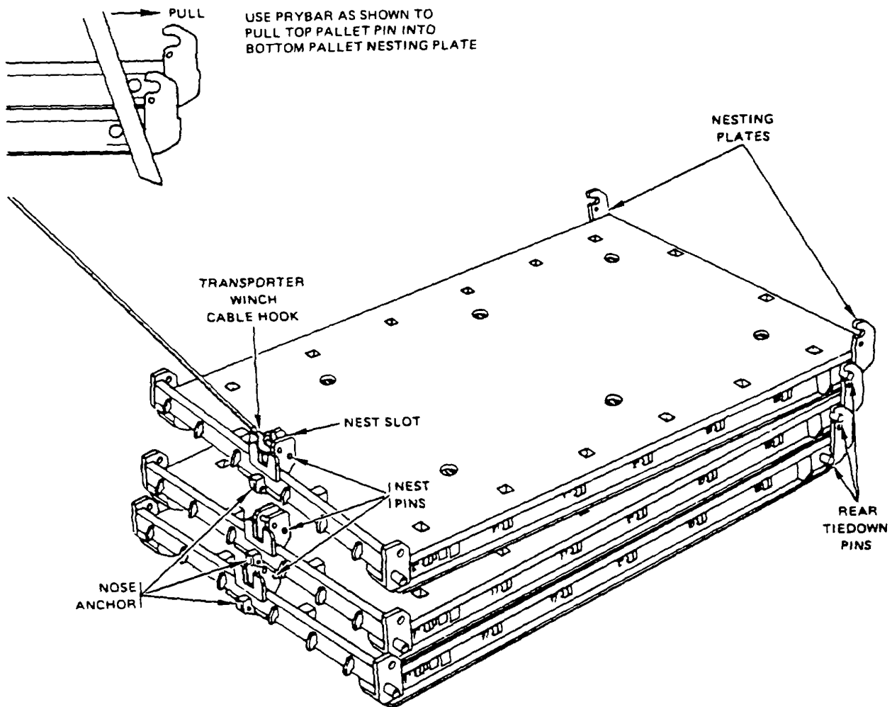
Figure 2-5. Nesting Pallets.
